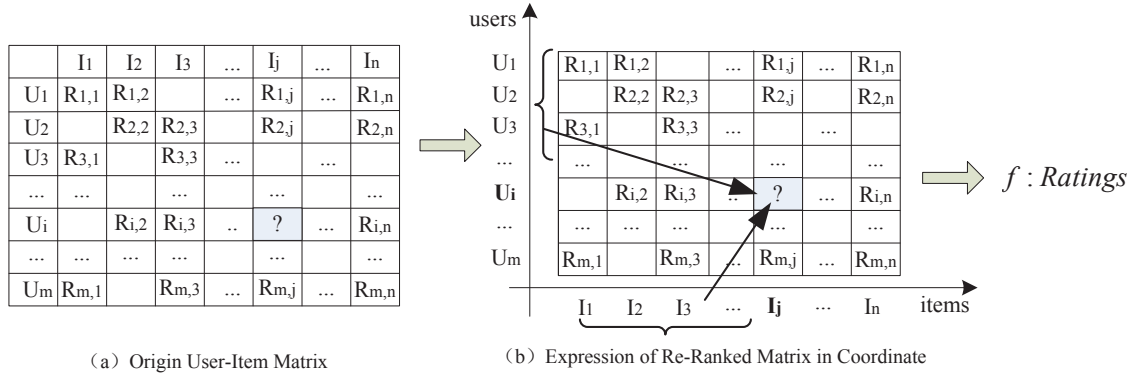
Figure 2: Principle of Predicting Rating Based on UICBF-I.
